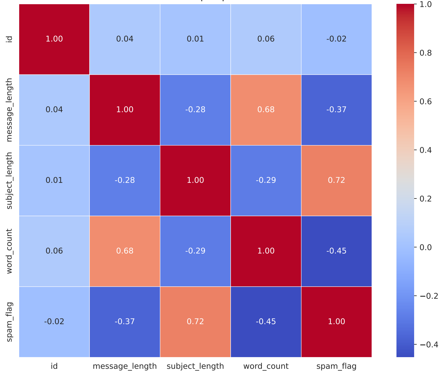
Correlation Heatmap - Spam Dataset
