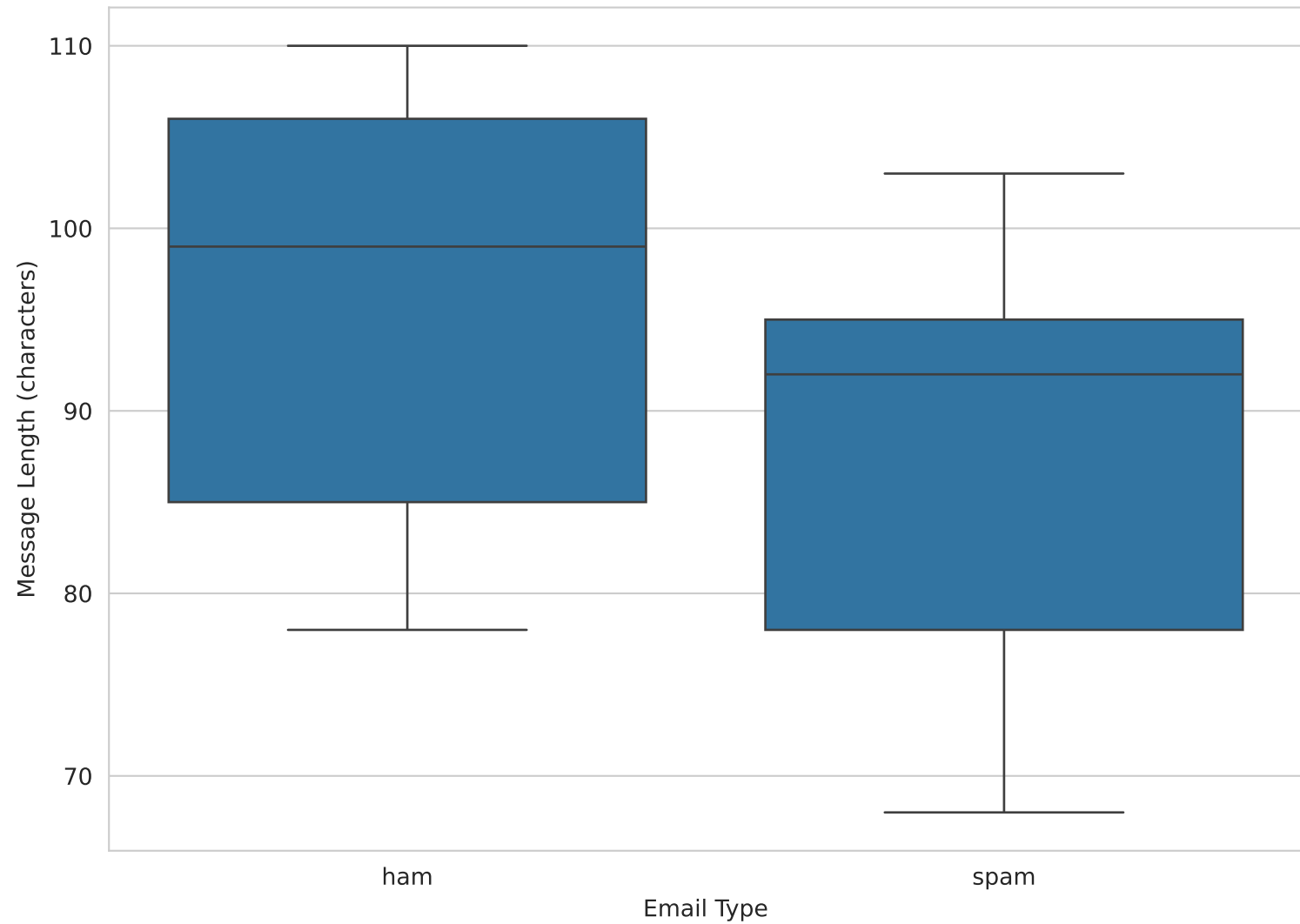
Message Length Distribution by Email Type
